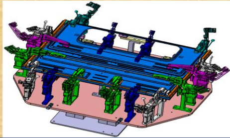
Rearwall & Assy Fixture
