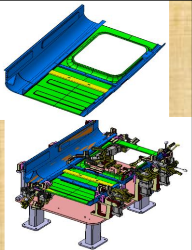
Corner Panel & Assy Fixture
