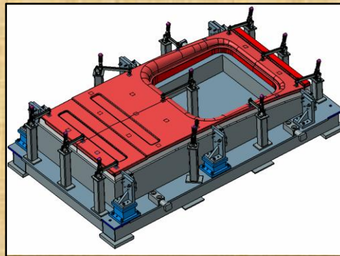
Side wall Panel Checker
